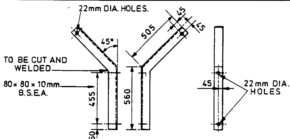
DETAIL OF CROSSARM BRACKET (SUPPLIED IN PAIRS)
